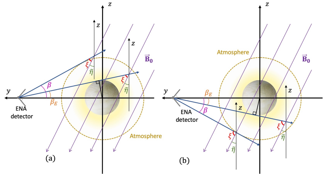
Figure 12. Schematic exemplifying the asymmetric range of angles \xi (red) between \mathbf{B}_0 and a LOS extended from the sub-Jovian detector (Figure 11e) into the northern (panel (a)) and southern (panel (b)) half spaces, shown in the x = 0 plane. Magnetospheric field lines projected into the x = 0 plane are presented in purple, with the tilt angle of \tilde{\eta} = 28.5^\circ against the (-z) axis represented in green. The detector is again conveyed by the gray line segments, and the upper boundary of Europa's atmosphere in the model is indicated by the dashed yellow circle. The maximum angle \beta (magenta) and minimum angle \beta_E (orange) between the boresight vector and a LOS outside of Europa's disc are also included.
