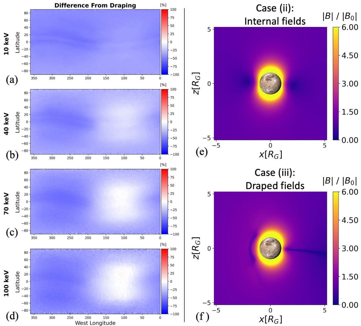
Figure 7. Influence of Ganymede's plasma interaction on the energetic neutral atom (ENA) emissions. Panels (a–d) illustrate the percent difference between the ENA flux recorded on the spherical detector for cases (ii) and (iii), that is, the percent change in the ENA flux through every location on the detector when the plasma interaction is included. Panels (a–d) were calculated by subtracting the flux maps in the center column of Figure 1 or Figure 2 from those in the right column. Each panel is arranged in the same way as the panels of Figure 1, with latitude on the vertical axis and West Longitude on the horizontal axis. The colorbar in panels (a–d) ranges from -100\% (blue) to +100\% (red). Thus, blue indicates locations where draping reduces the ENA flux, and any (faint) red represents locations where draping enhances the ENA flux. Panels (e, f) show the magnetic field magnitude |B| in the y = 0 plane for cases (ii) and (iii), respectively. The values of |B| in panels (e, f) are normalized with the ambient Jovian field magnitude |B_0| = 80.2 nT (see Section 2.1), and the axes are scaled in units of R_G .
