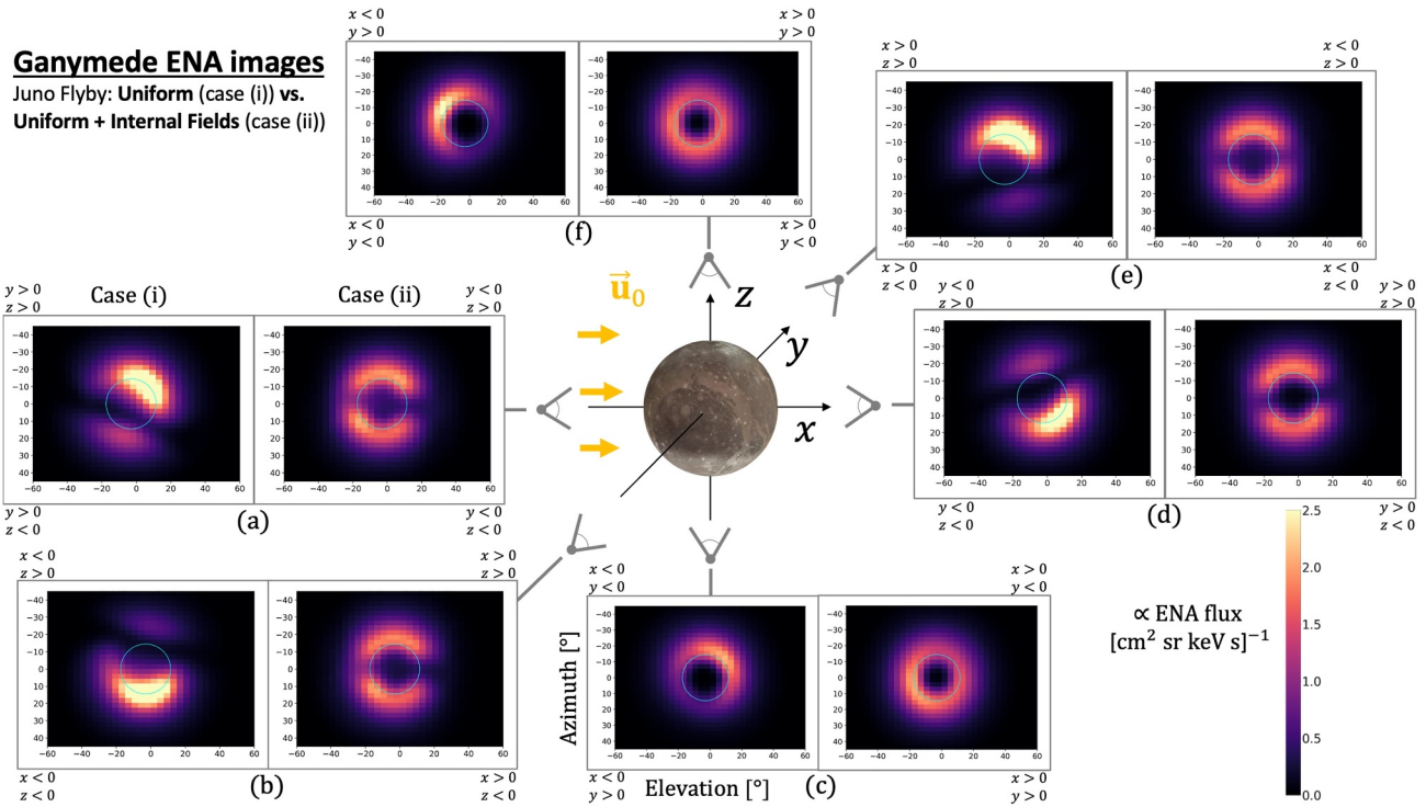
Figure 9. Synthetic energetic neutral atom (ENA) images, calculated for uniform fields (case (i)) and Ganymede's internal field superimposed with the ambient Jovian field (case (ii)) on the left and right sides of each panel, respectively. The ENA images are arranged with detector elevation on the horizontal axis and detector azimuth on the vertical axis. Ganymede's disc is illustrated by the blue circle in each subplot. The direction of the upstream plasma flow \vec{u}_0 is represented by the yellow arrows. For each synthetic ENA image, the detector is located at |\vec{r}| = 4R_G , and the boresight vector points radially towards the center of Ganymede. The gray symbol connected to every panel represents the detector, pointing at the moon with its boresight vector parallel or antiparallel to a coordinate axis of the GPhiO system. In panels (a, d), the detectors are located along the x axis at (\pm 4R_G, 0, 0) with the boresight vectors (\pm 1, 0, 0) . In panels (b, e), the detectors are positioned on the y axis at (0, \pm 4R_G, 0) with boresight vectors of (0, \pm 1, 0) . In panels (c, f), the detectors are positioned along the north-south axis at (0, 0, \pm 4R_G) with boresight vectors given by (0, 0, \pm 1) . The labels in the corners of each image denote which quadrants of the GPhiO system are visible in the quadrants of the images. The values of the ENA flux for our chosen timestep (see Section 2.3 and Haynes, Tippens, et al., 2025) are given by the colorbar in the lower-right corner.
