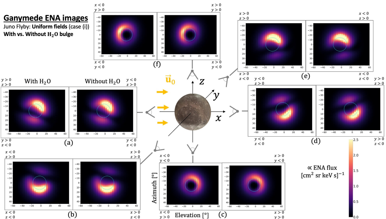
Figure A1. Synthetic energetic neutral atom images of Ganymede's magnetosphere-atmosphere interaction in uniform fields (case (i)), with (left) and without (right) the presence of the H 2 O atmospheric component. The figure is arranged in the same way as Figures 9 and 12.
