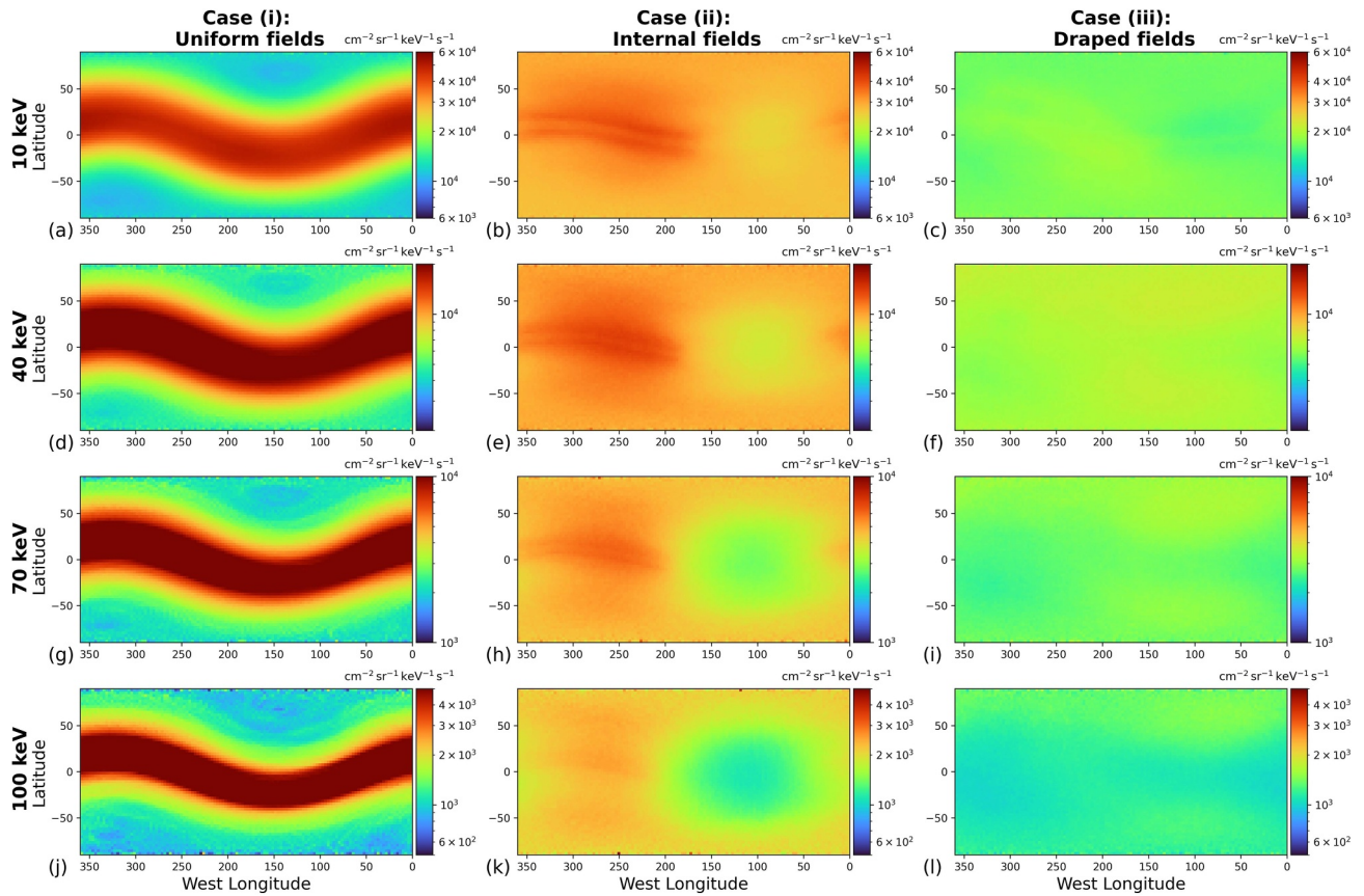
Figure 2. Global maps of energetic neutral atom flux emanating from Ganymede's atmosphere, identical to those displayed in Figure 1, but with a different range of the colorscale in each row to reveal fine structures in the emission morphology. The figure is organized in the same manner as Figure 1. The colorscale is logarithmic, with its range changing from row to row. The minimum and maximum values in each row are always one order of magnitude apart.
