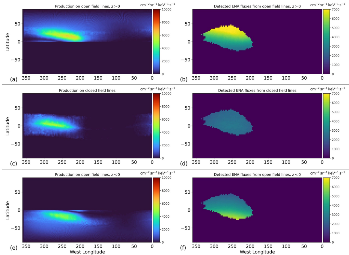
Figure 6. Connection between production and detection of energetic neutral atoms (ENAs) from the “stripe” features. The panels in the left column display the decomposition of ENA production by longitude and latitude (see Figure 5). However, the “dual stripe” feature from Figure 5(a) is now separated into the contributions from the northern ( z > 0 , panel (a)) and southern ( z < 0 , panel (e)) hemispheres. ENA production on closed field lines is illustrated in panel (c), which is identical to Figure 5(b). The three panels in the right column illustrate the contributions of these three production regions to the flux through the patch on the detector sphere at |r| = 3R_G : (b) detected flux from the northern stripe, (d) flux observed from the central stripe, and (f) flux produced in the southern stripe.
