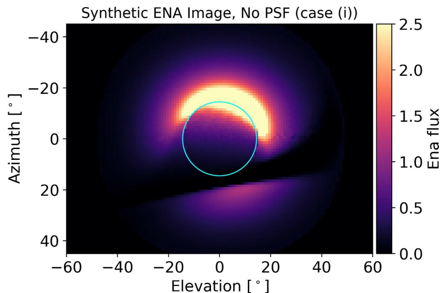
Figure 10. Synthetic energetic neutral atom (ENA) image at Ganymede for case (i), captured by the detector above the sub-Jovian apex, without the point spread function or the downscaling procedure applied. After the post-processing steps, this synthetic ENA image would become the same as the left subplot in panel 9(e).
