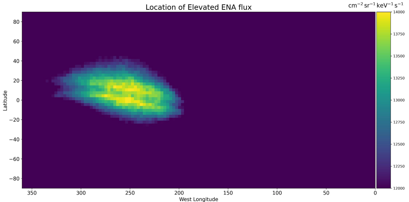
Figure 3. Energetic neutral atom (ENA) flux recorded on the spherical detector for a superposition of Ganymede's internal field and the Jovian magnetospheric field (case (ii)) and at an initial parent proton energy of 40 keV. The vertical and horizontal axes represent latitude and West Longitude, respectively. This flux map is identical to those shown in Figures 1e and 2e. However, a linear colorscale is used, with its lower edge chosen to facilitate the identification of a “patch” of elevated ENA flux in the emission pattern on the detector. For this purpose, pixels with ENA fluxes below 12,000 \text{ [cm}^2 \text{ sr keV s]}^{-1} (the minimum value on this scale) appear purple. Fluxes above this threshold define the feature under investigation and appear in yellow, green, and blue. Only locations on the detector with fluxes above 12,000 \text{ [cm}^2 \text{ sr keV s]}^{-1} are included in our subsequent analysis of the associated parent proton population.
