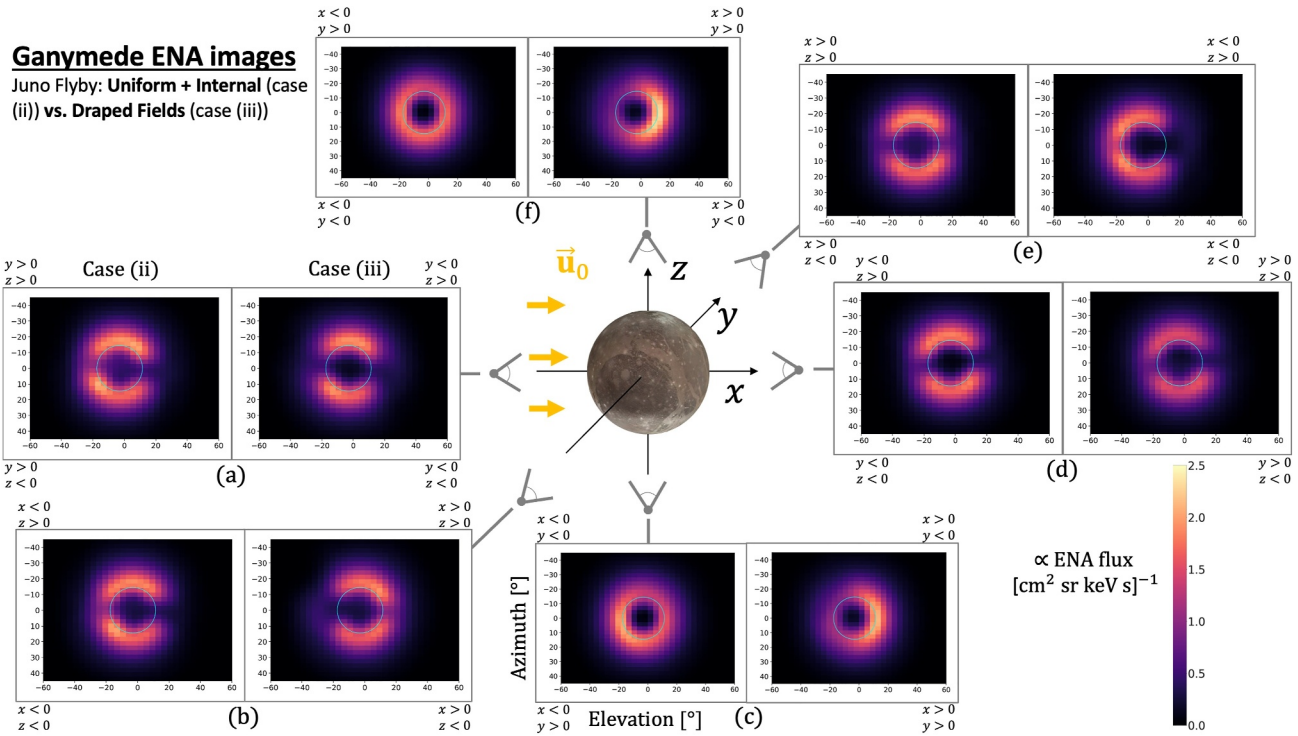
Figure 12. Synthetic energetic neutral atom (ENA) images of Ganymede's mini-magnetosphere, without (case (ii)) and with (case (iii)) draped fields from AIKEF included. The layout of the figure is the same as that of Figure 9. The images for cases (ii) and (iii) are shown on the left and right side of each panel, respectively. To facilitate comparison between cases of successively increasing complexity, the synthetic ENA images on the left side of the panels in this figure are the same as those on the right side of the respective panels in Figure 9. For all panels (a–f), detector elevation is on the horizontal axis and detector azimuth is on the vertical axis. In each image, Ganymede's disc is represented by the blue circle. The detector is positioned at a distance of |\mathbf{r}| = 4R_G . The corners of every panel are labeled according to the quadrants of the GPHiO System. The gray detector symbol attached to each panel illustrates the viewing geometry in the respective images. The range of the colorscale and the time step used for these images are the same as in Figure 9.
