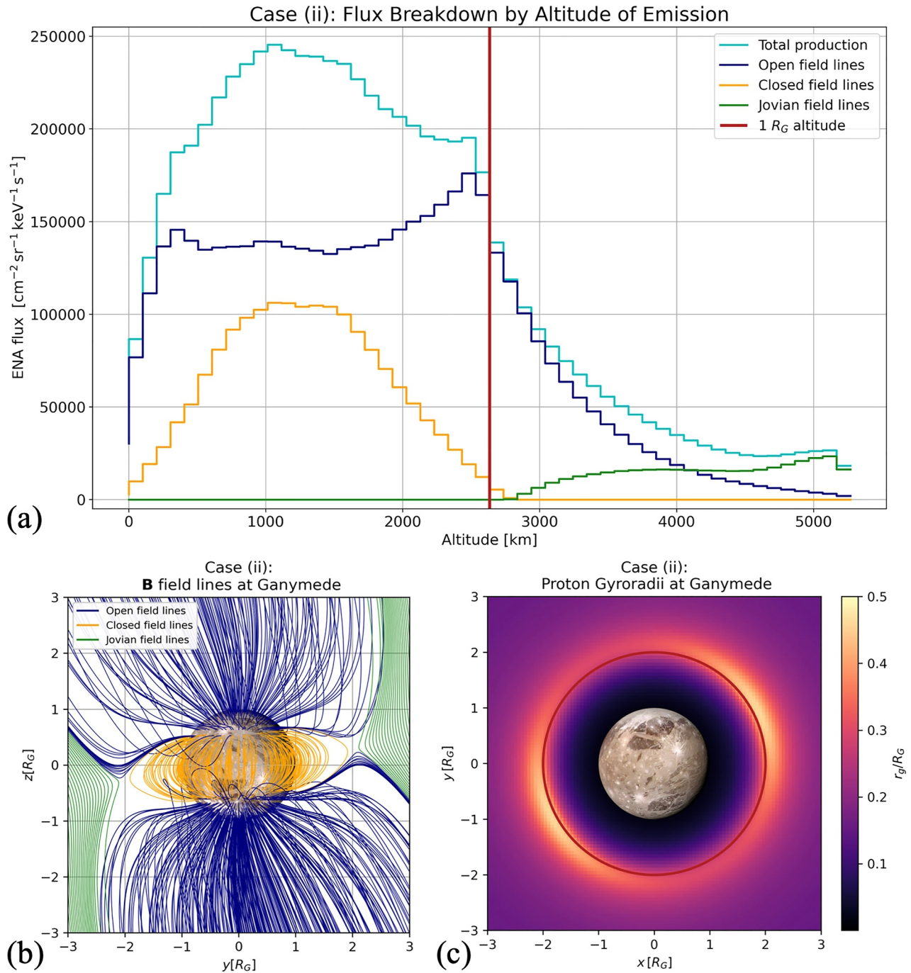
Figure 4. Relation between energetic neutral atom (ENA) emissions and the magnetic field topology near Ganymede. For case (ii), panel (a) provides an altitude profile of the generation region for the ENA flux emitted toward the “patch” feature identified in Figure 3. The histogram is computed by grouping the ENA flux generated by the contributing 40 keV protons into altitude bins of approximately 100 km height, irrespective of the longitude and latitude of ENA production. The horizontal axis displays the altitude above Ganymede’s surface, and the vertical axis represents the locally produced ENA flux. Panel (a) takes into account the points of origin for all ENAs contributing to the patch feature. The total ENA production within each altitude bin is shown in cyan. The plot also identifies the ENA populations emanating from protons on “closed” field lines that connect to Ganymede at both ends (orange curve), “open” field lines that connect Ganymede’s internal field to Jupiter’s field (navy curve), and Jovian magnetospheric field lines which do not connect to the moon (green curve). The vertical red bar corresponds to an altitude of 1 R_G . It is emphasized that panel (a) does not show the locations where ENA flux is being recorded. Panel (b) illustrates the magnetic field topology near Ganymede for case (ii). Field lines are depicted in the x = 0 plane, that is, in a cut perpendicular to the incident flow \mathbf{u}_0 . The field lines are colored analogous to panel (a): open field lines are navy, closed field lines are orange, and Jovian field lines are green. Also for case (ii), panel (c) depicts a map of the local 40 keV proton gyroradii near Ganymede in the equatorial ( z = 0 ) plane. A pitch angle of \alpha = 90^\circ was assumed to generate this plot. The colorscale ranges from r_g = 0 to r_g = 0.5 R_G \approx 1,317 \text{ km} . The dark red circle corresponds to an altitude of 1 R_G .
